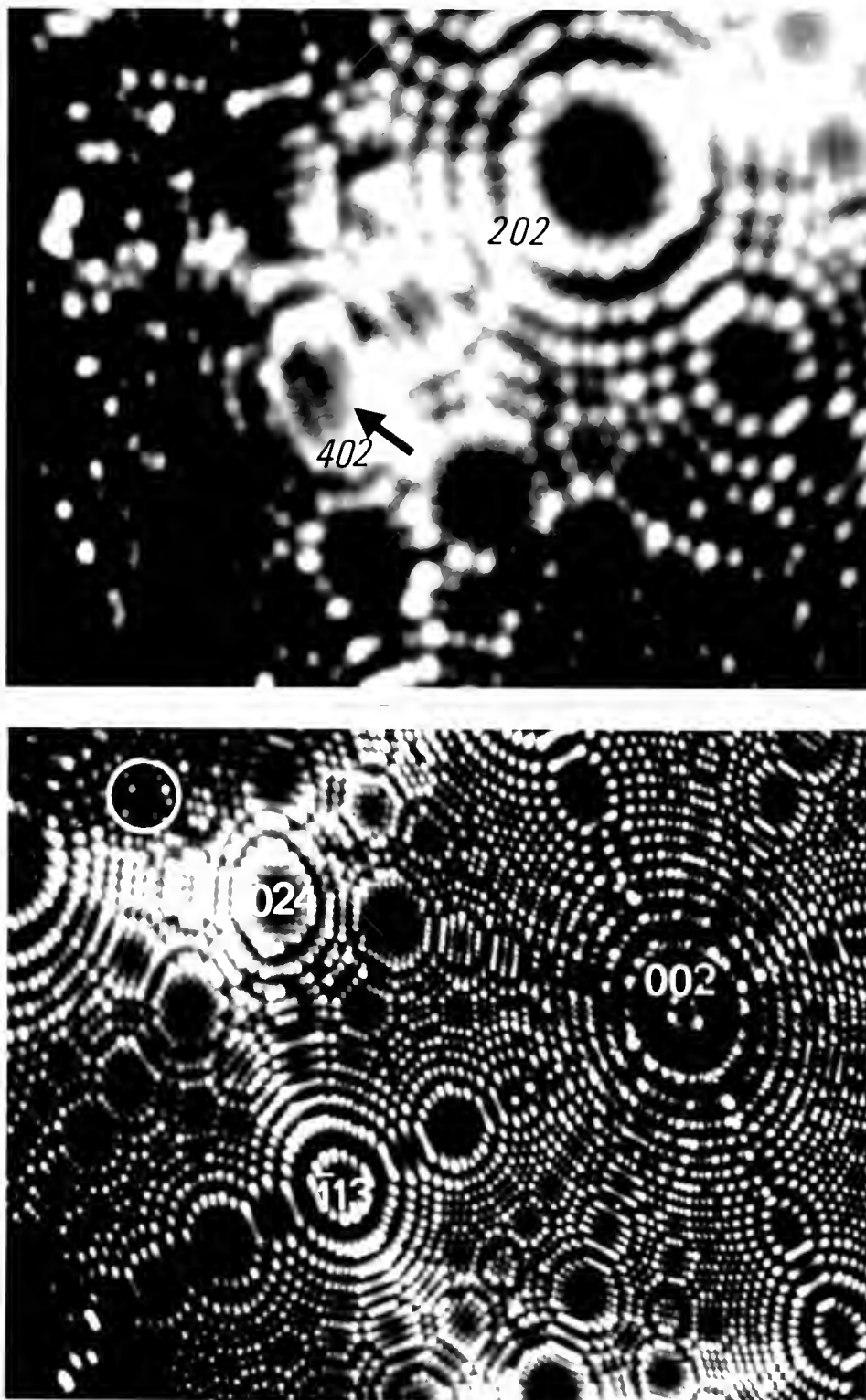
Figure 37.--Field ion micrographs of vacancy clusters in platinum. (a) An irregular cluster on a {420} plane. (b) A tetrahedral cluster near {220} plane. Both defects are about 25 Å in diameter.
